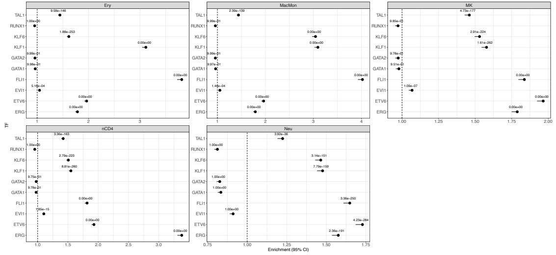
S14 Fig. Transcription factor motif enrichment analysis for (A) SIPs versus non-SIPs. (B) SIP PIRs versus non-SIP PIRs. The Y-axis shows the transcription factor and X-axis shows odds ratio of enrichment. The dot denotes the point estimate of odds ratio and the line denotes the lower 95% confidence.
