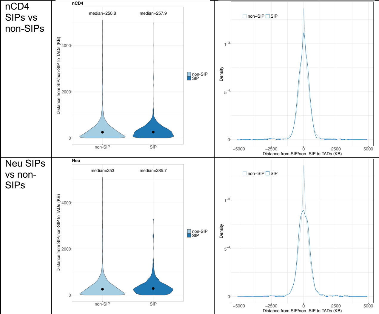
S15 Fig. Distance to TAD boundary for SIPs versus non-SIPs. Distributions of distance to TAD boundaries for non-SIPs versus SIPs are visualized using side-by-side violin plots (left) and overlapping density plots (right).
