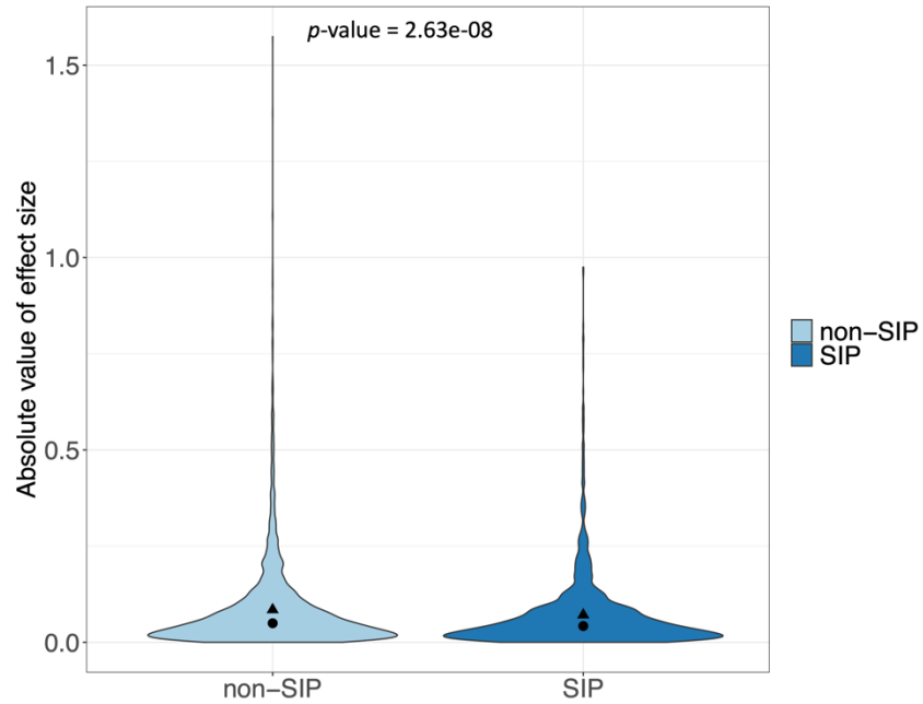
S25 Fig. Effect size when perturbing PIRs, SIPs versus non-SIPs. Effect sizes are from CRISPRi experiments in Gasperini et al[1]. Dots denote median, and triangles denote mean.
