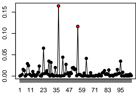
cook.d
