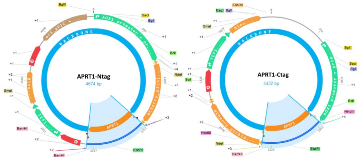
S1 Fig. Vector maps of APRT1-Ntag (left) and APRT1-Ctag (right). P. pastoris expression vector pPICZ maps, showing the aprt1 gene insert position, and location of mCherry tags.
