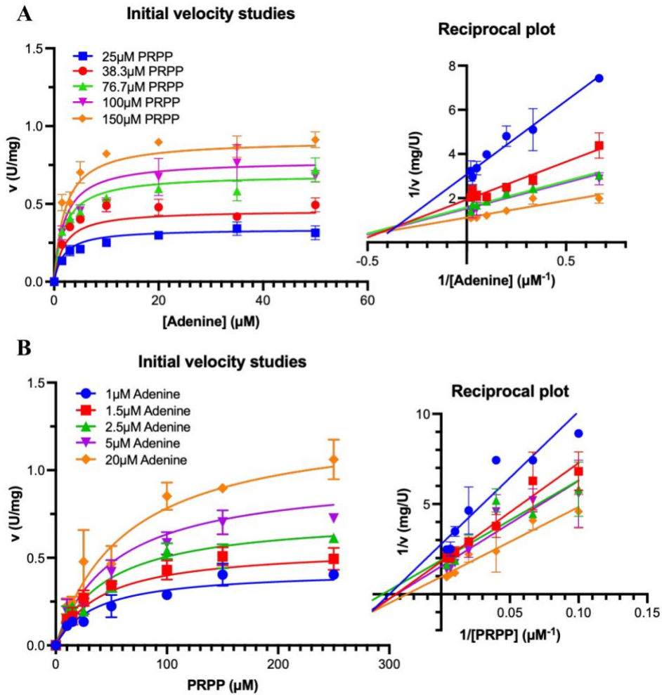
S6 Fig. Bi-substrate kinetics of APRT1 forward reaction. (A) Initial velocities of APRT1 at fixed-changed PRPP concentrations, varying substrate adenine. (B) Initial velocities of APRT1 at fixed-changed adenine concentrations, varying substrate PRPP. Data Insets shows double reciprocal plots of A and B.
