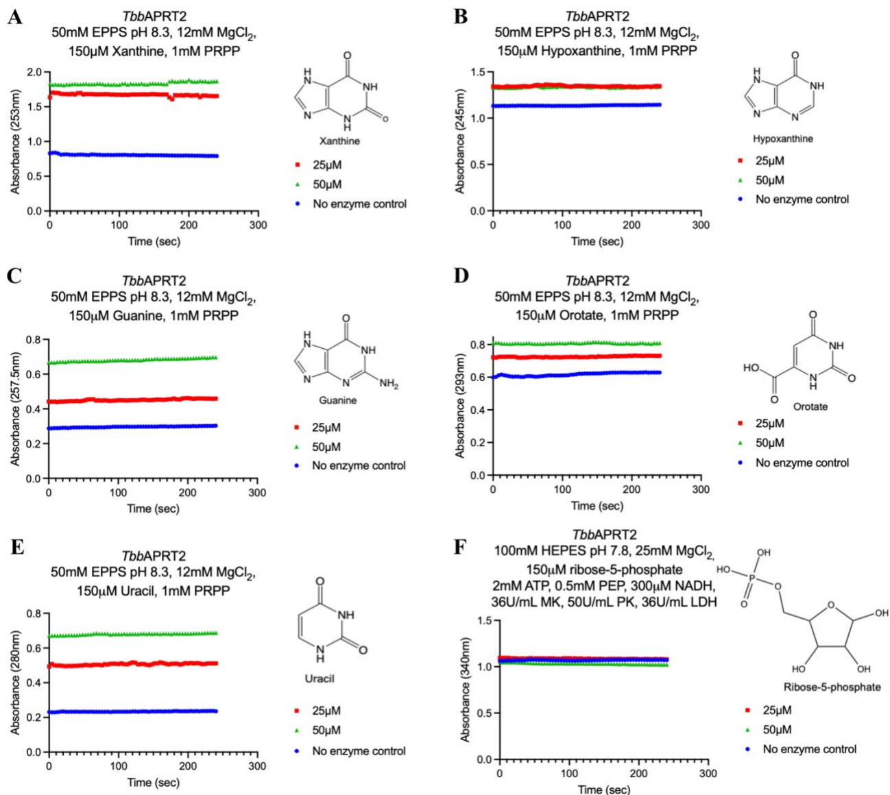
S12 Fig. APRT2 Type 1 PRTase activity tests using alternative N-containing nucleophiles – part 1. APRT2 was tested for activity as a potential HGXPRT, EC 2.4.2.8 (A, B, C); OPRT, EC 2.4.2.10 (D), UPRT, EC 2.4.2.9 (E), and PRPP synthetase, EC 2.7.6.1 (F). No enzymatic activity could be detected under the assay conditions described in the Methods.
