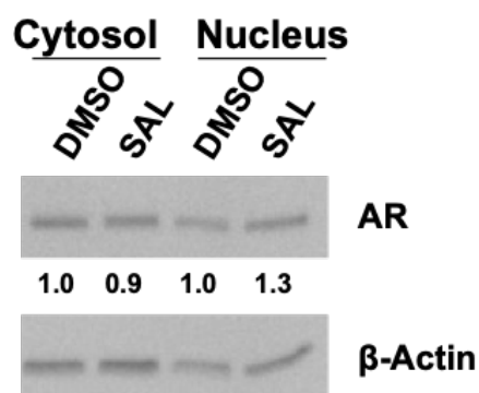
Fig. S3. Protein levels of AR in cytosol and nucleus. LNCaP cells were lysed after 24 h treatment with SAL and DMSO and separated into cytosolic and nuclear protein fractions. Western blot was performed to analyze AR levels. Values of control samples were set arbitrarily as 1. Quantification of bands was performed by LabImage D1 normalized to the loading control \beta -Actin.
