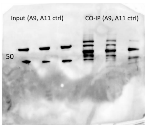
Supplementary Figure S3. Hsp70 interacts with PKA-C \alpha in A9 and A11 cells. (a) Hsp70 expression is demonstrated in all cell lines. Following co-immunoprecipitation with PKA-C \alpha antibody, Hsp70 is identified in the protein complexes from A9 and A11. (b) Full-length blot represented in panel A.
