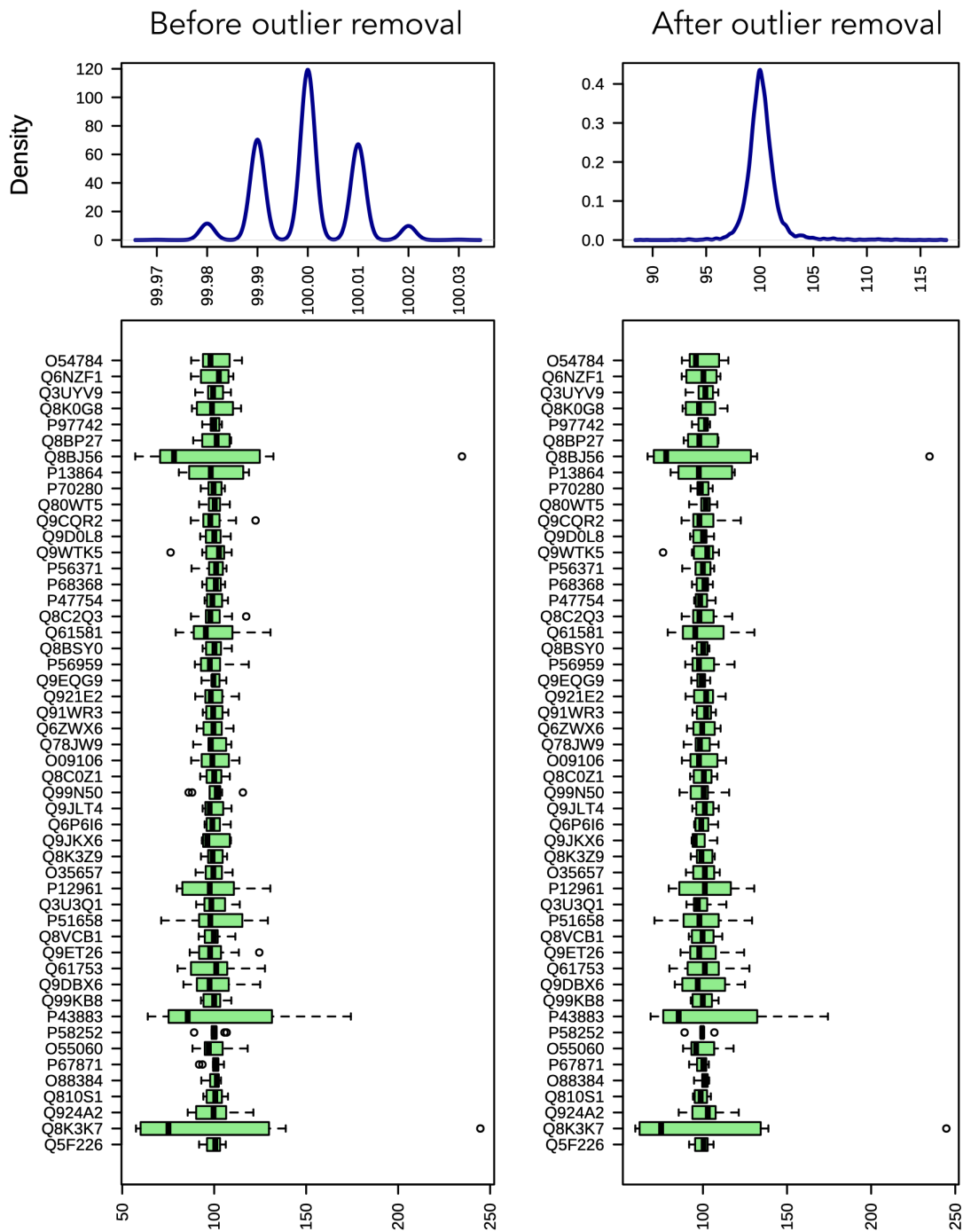
Box plots and kernel density plots before ( n=10 ; Cases=5, Controls=5) and after ( n=8 ; Cases=4, Controls=4) removal of outliers from dataset. The boxplots show a maximum of 50 proteins due to space limit. The density plots are based on all samples before and after outlier removal.
