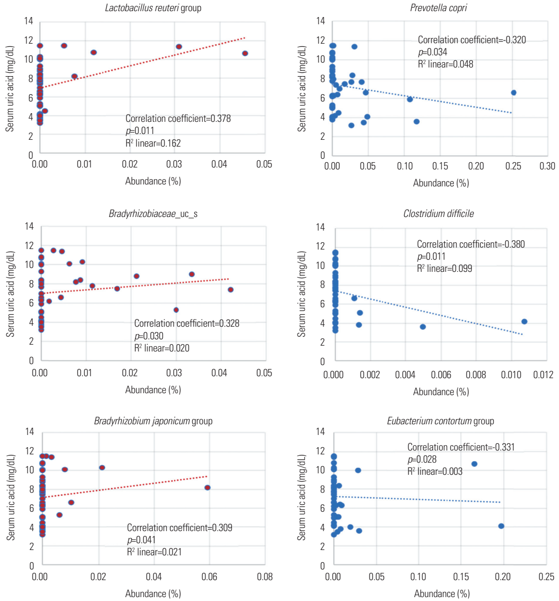
Supplementary Fig. 4. Nonparametric Spearman correlation between serum uric acid level and abundance of microbiota.
