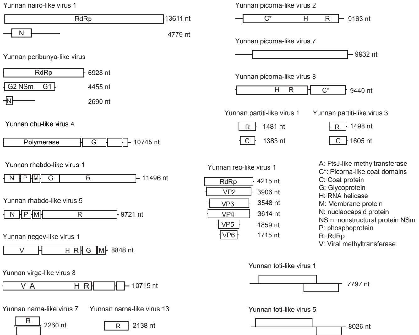
Figure S1. Representative genome organizations of the viruses with (nearly) complete genomes carried by arthropods on the body surface of bats. The genomes are drawn to a unified length scale. Predicted ORFs of these genomes are labeled with information on the potential protein or protein domain that they encode.
