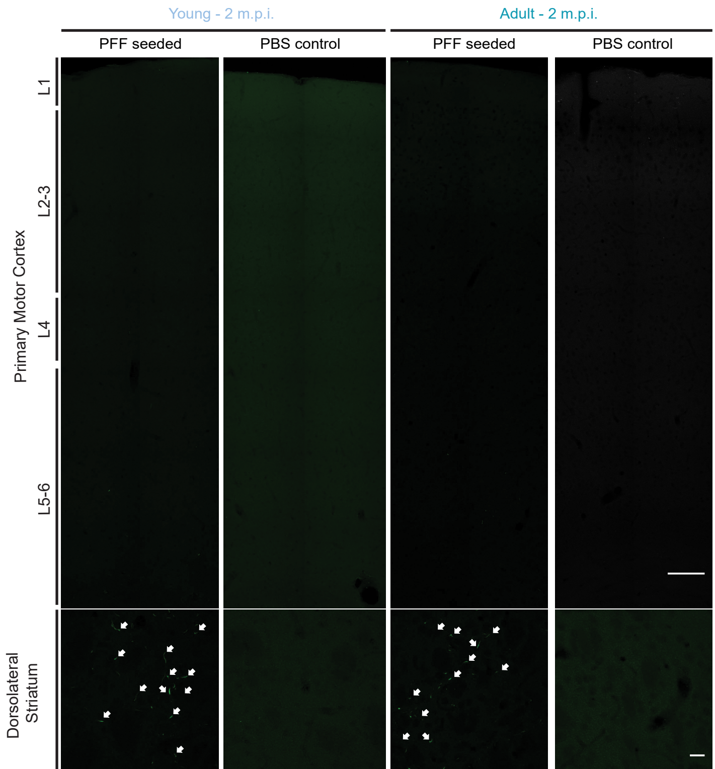
Figure S2. Spreading of alpha-synuclein from the SNpc did not reach the motor cortex 2 months after PFFs inoculation. Phospho- \alpha -synuclein (pSyn) staining in primary motor cortex and striatum acquired from the same coronal slice in young and adult mice, 2 m.p.i.. Immunoreactivity of pSyn-positive aggregates was observed only in the striatum ipsilateral to the PFFs injection. This observation validates our experimental design that use the contralateral hemisphere as internal control. Scalebar 50 \mu m.
