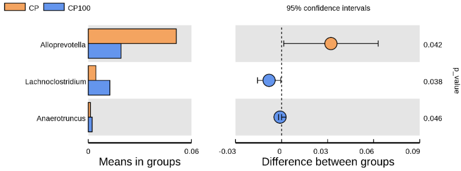
Figure S5. T-test results of species differences on genus level between groups. CP was the CY group, CP100 was the CY+CPPF-M group; N=7.
