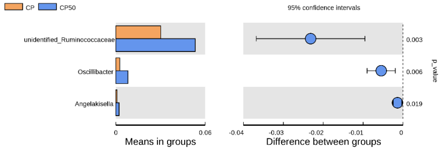
Figure S4. T-test results of species differences on genus level between groups. CP was the CY group, CP50 was the CY+CPPF-L group; N=7.
