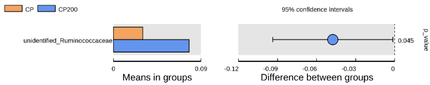
Figure S3. T-test results of species differences on genus level among groups. CP was the CY group, CP200 was the CY+CPPF-H group; N=7.
