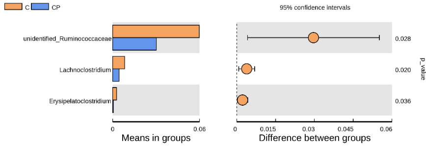
Figure S1. T-test results of species differences on genus level between groups. C was the Control group, CP was the CY group; N=7.
