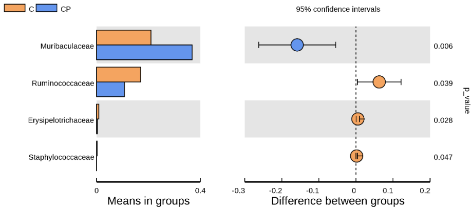
Figure S2. T-test results of species differences on family level between groups. C was the Control group, CP was the CY group; N=7.
