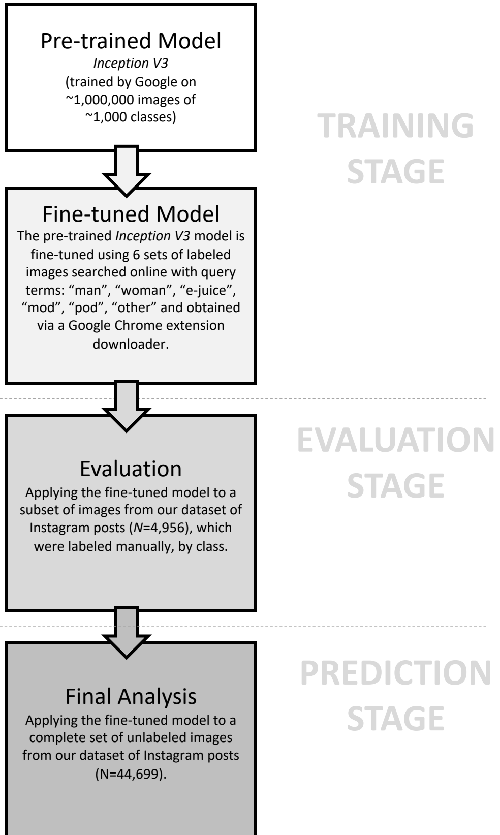
Supplementary Figure 4. Training, evaluation and prediction stages for deep learning image classification.
