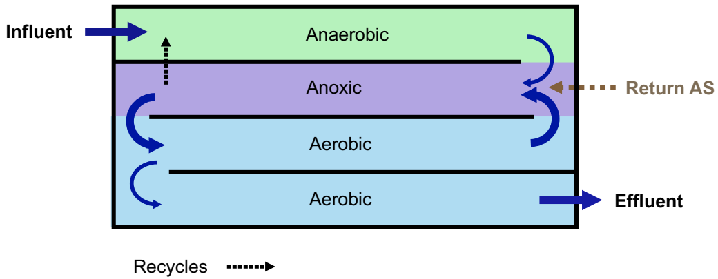
Supplementary Figure S1. Schemes of two types of bioreactors operated using the UCT technology.
