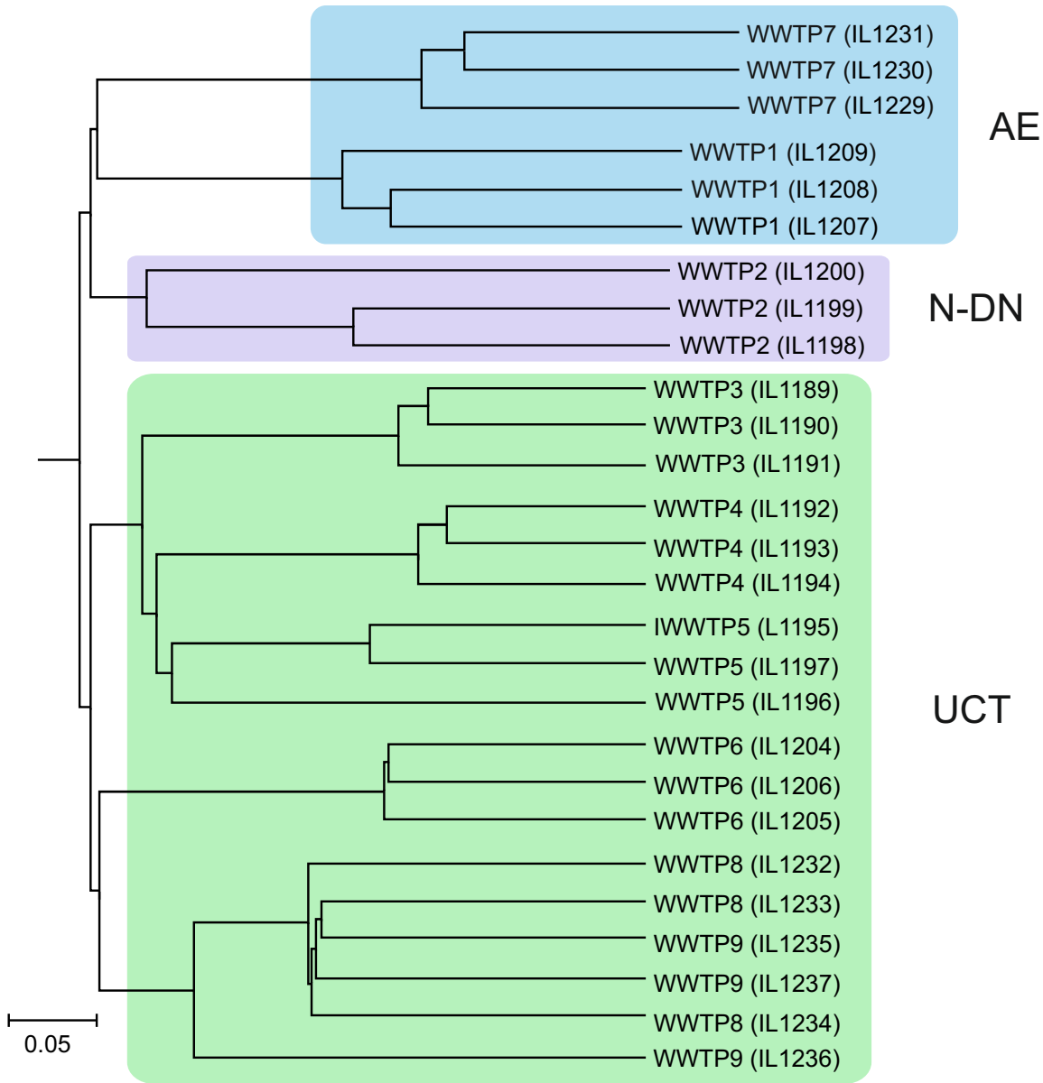
Supplementary Figure S2. Neighbor joining tree illustrating Jaccard distances between microbial communities of AS samples from 9 WWTPs (three replications). Sample IDs are shown in brackets after the WWTP number.
