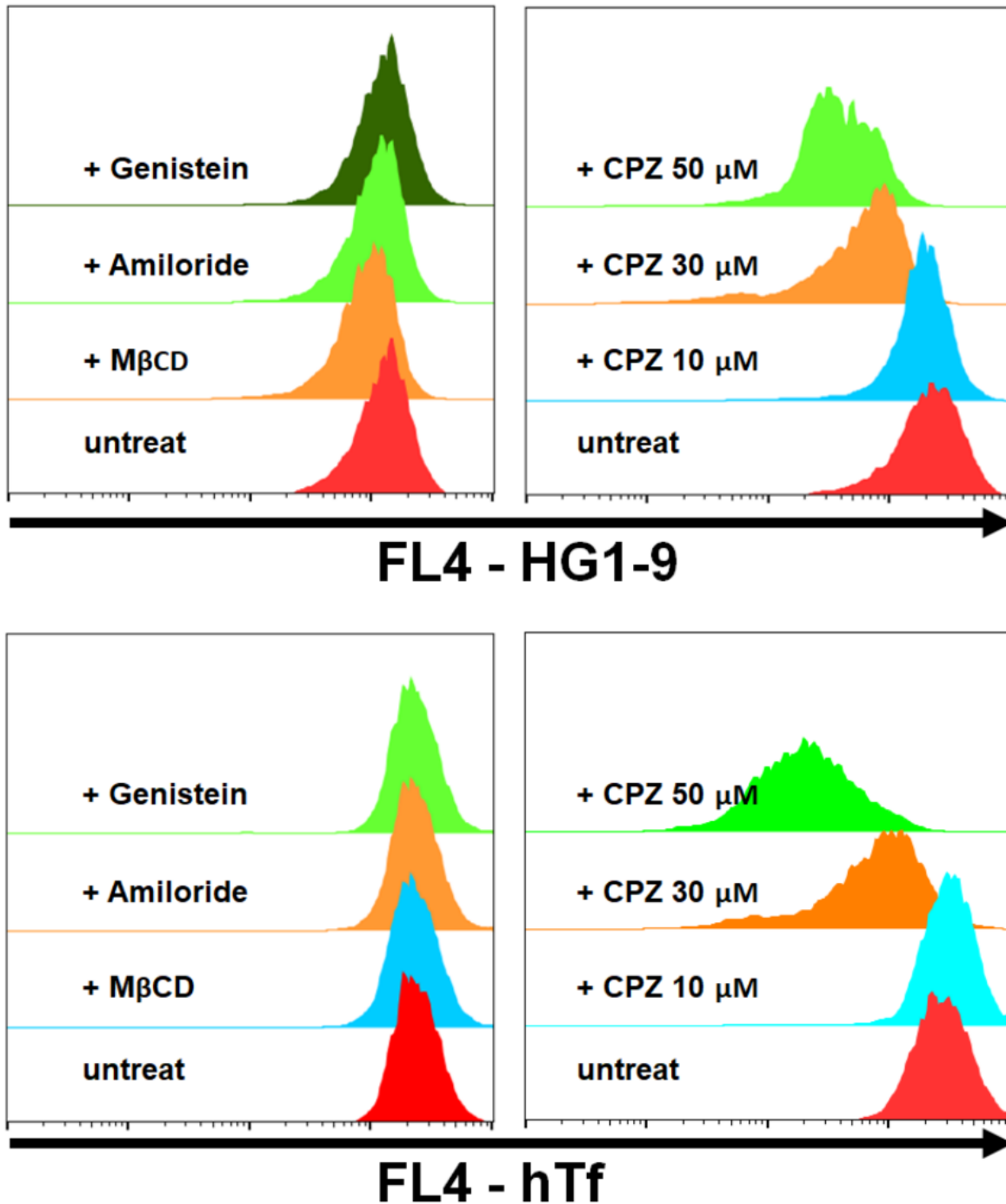
Figure S2. Flow cytometry analysis of the uptake of aptamer HG1-9 and hTf (200 nM, labeled by AF647) by cells pre-treated with endocytosis inhibitors (50 μM Amiloride, 50 μM Genistein and 5 mM Methyl-β-cyclodextrin (MβCD); Chlorpromazine (CPZ, 10, 30 and 50 μM)); the uptake by untreated cells was as positive control; at least two independent experiments were done.
