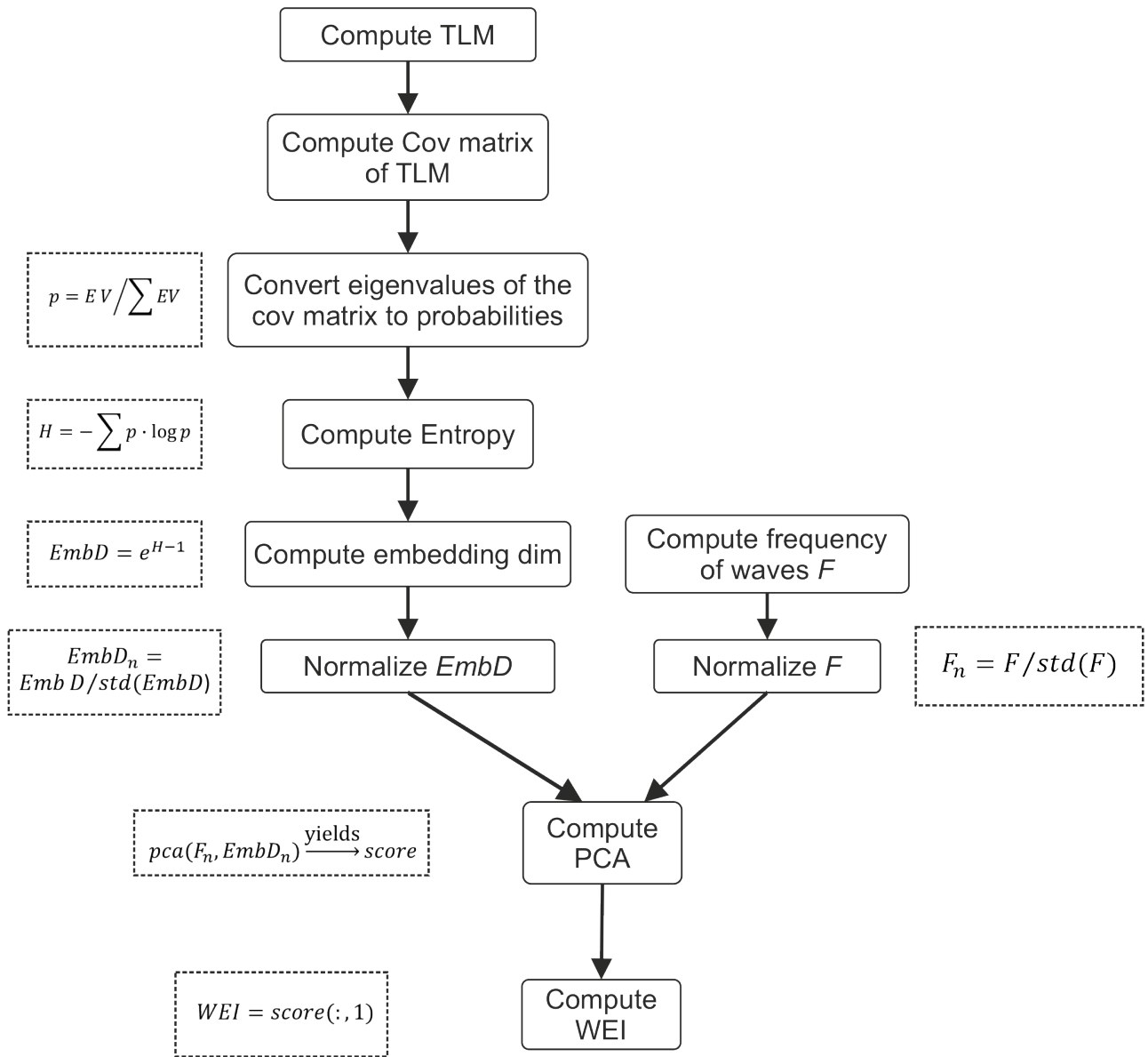
Figure S1: Schematic representation of the calculation of the wave entropy index (WEI), Related to Figs. 1-2 and to Section “Extraction of the wave entropy index (WEI)”.
