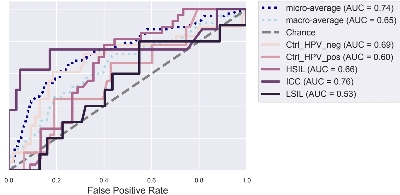
Per-Class Receiver Operating Characteristics
