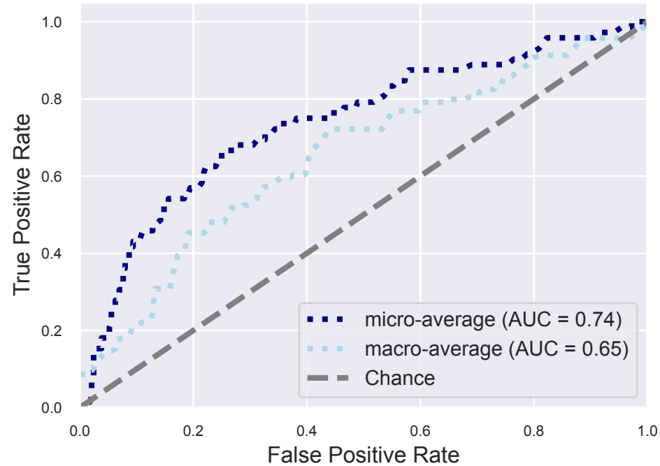
Receiver Operating Characteristic Average Scores
