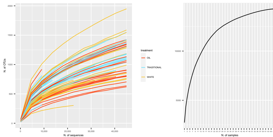
S1 Figure 1. Rarefaction curves. Sequence-based (left) and sample-based (right) rarefaction curves for the sampled gut microbiotas. Number of detected OTUs on the y-axis; number of sequences (left) and of samples (right) on the x-axis.
