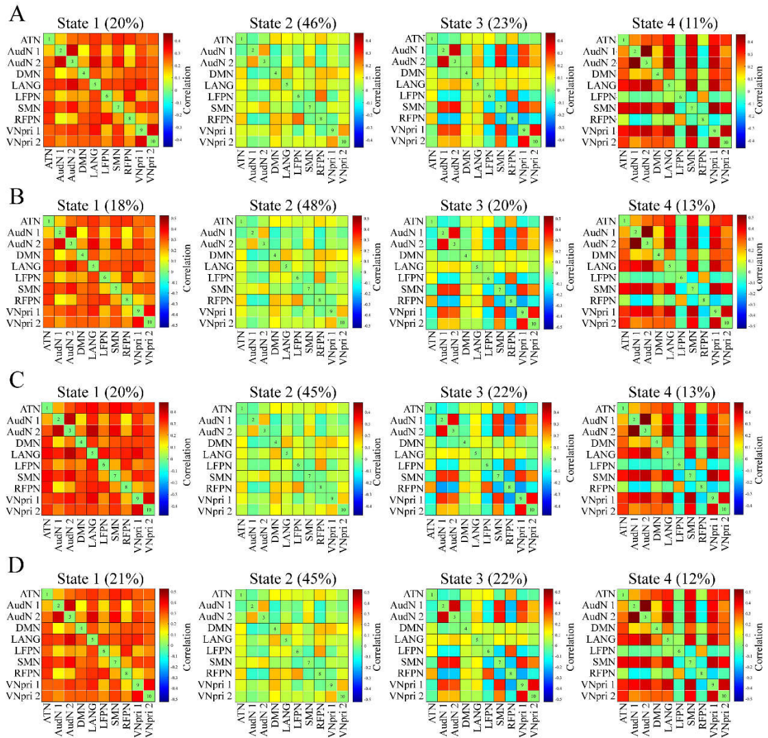
Fig S1. Validation test about the influence of Gaussian window alpha value ( \sigma ) on dFNC states. (A) Four dFNC states in the main text, the \sigma was 3 TRs, and the window size was 25 TRs. (B) Four dFNC states when the \sigma was 1 TRs, and the window size was 25 TRs. (C) Four dFNC states when the \sigma was 3 TRs, and the window size was 20 TRs. (D) Four dFNC states when the \sigma was 3 TRs, and the window size was 30 TRs. We can see that both the states and their frequencies were consistent.
