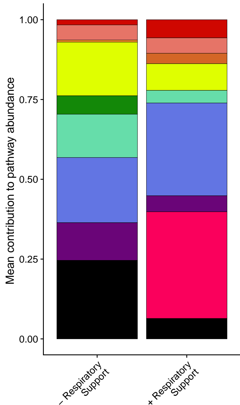
PWY-1269: CMP-3-deoxy-D-manno- octulosonate biosynthesis I
