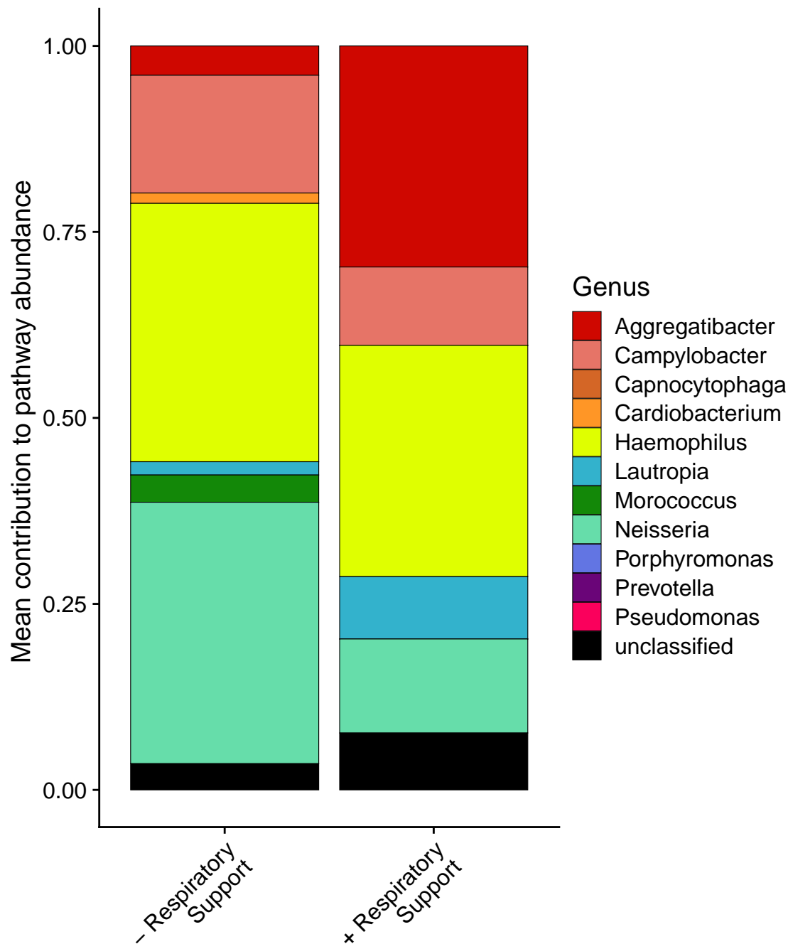
NAGLIPASYN-PWY: lipid IVA biosynthesis
