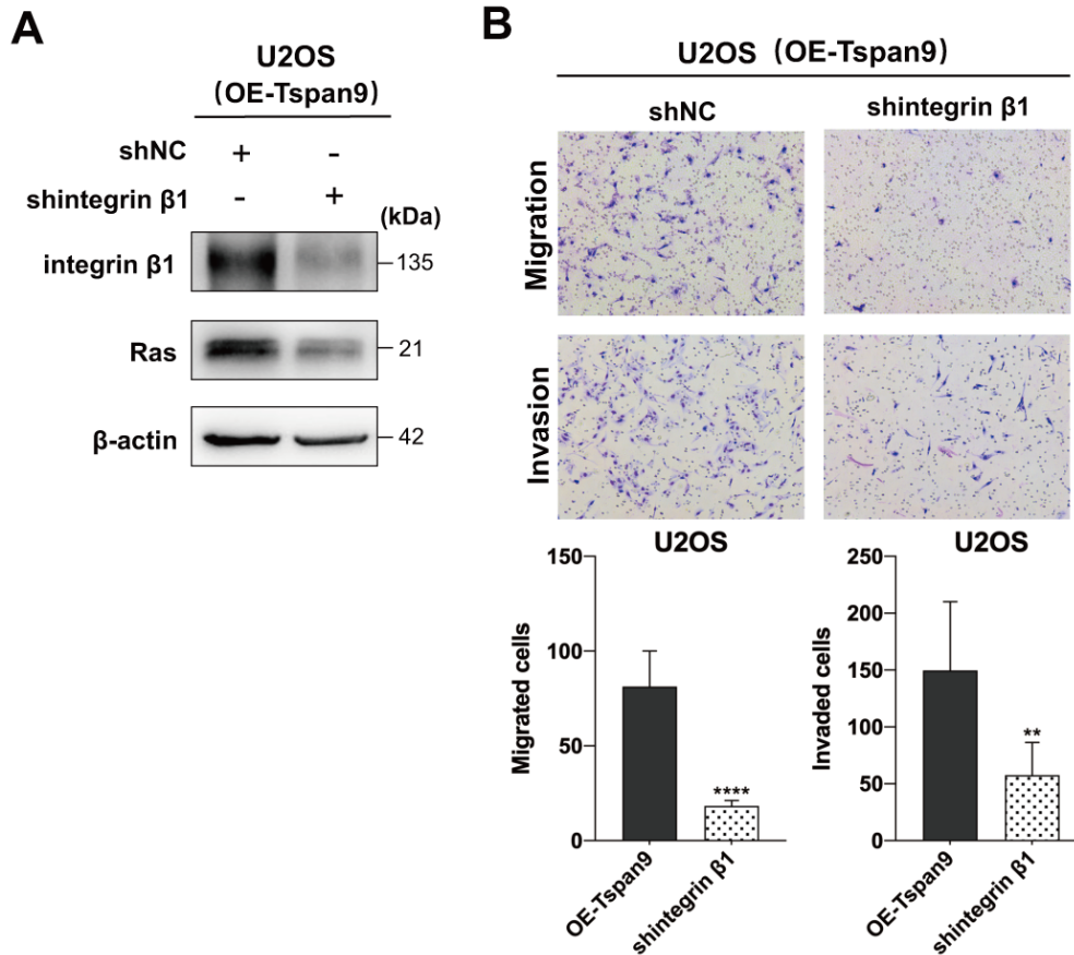
Figure S2. Knockdown of \beta 1 integrin inhibits downstream Ras expression and the metastasis of OS cells in vitro. (A) Knockdown efficiency of integrin \beta 1 in Tspan9-overexpression U2OS cells and regulation of downstream Ras were confirmed by Western blotting. (B) The impact of integrin \beta 1 knockdown on OS cell migration and invasion was assessed via a Transwell approach. All analyzes were repeated two or three times. Data are means \pm SD. ** P < 0.01 ; **** P < 0.0001 .
