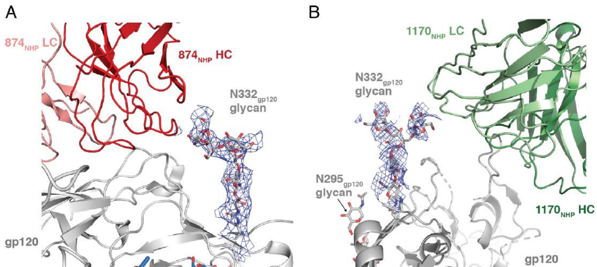
Figure S6. Antibodies Ab874 NHP and Ab1170 NHP interact with the N332 gp120 glycan. Antibodies (A) Ab874 NHP and (B) Ab1170 NHP elicited in NHPs after priming with RC1-4fill-VLPs (115) contact the high-mannose N-glycan attached to gp120 residue N332 (modeled from PDB 6ORO) (Ab874 NHP ) and this study (Ab1170 NHP ). Cryo-EM density for the N332 gp120 glycan is shown as blue mesh contoured at 4σ.
