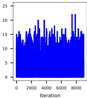
Number of non-ancestral recomb
