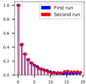
Autocorrelation
