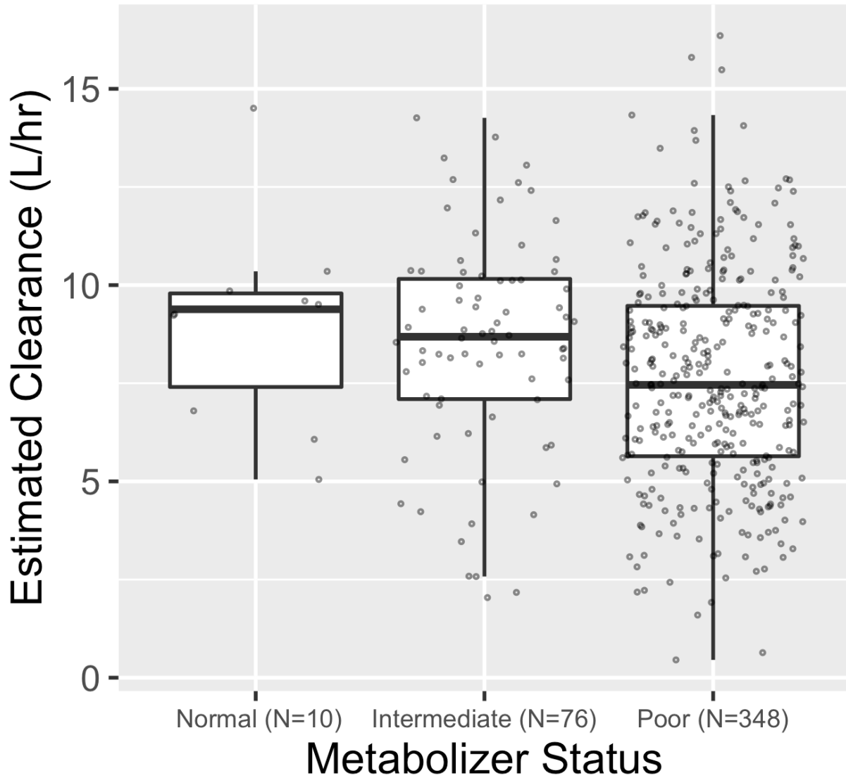
Figure S1: Individual estimated clearance by CYP3A5 metabolizer status standardized at 7.7kg. Estimated clearance at 7.7kg is calculated for each individual and summarized for normal, intermediate, and poor metabolizers. The hinge is set at the median, the boxes span the 25 th to 75 th percentile, the whiskers extend to the most extreme datum which is at most 1.5 times the distance from the interquartile range.
