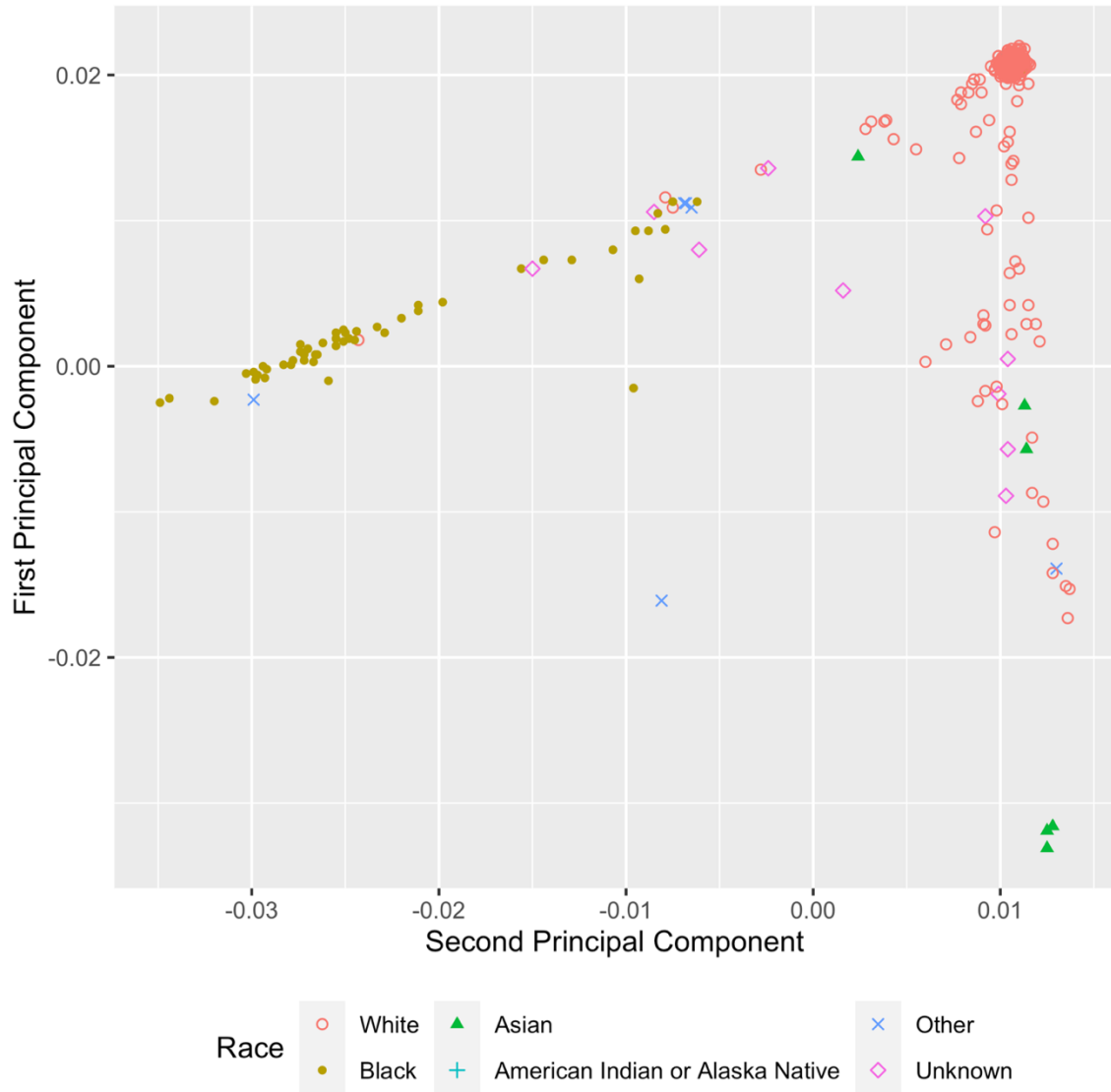
Figure S2: Principal components for ancestry informative markers. Axes correspond to values for the first and second principal components. Self-reported race is specified by point color.
