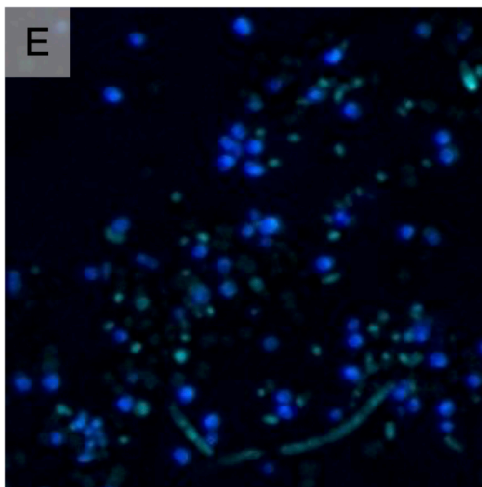
Overlay Alphaproteobacteria + Verrucomicrobia-Plancto
