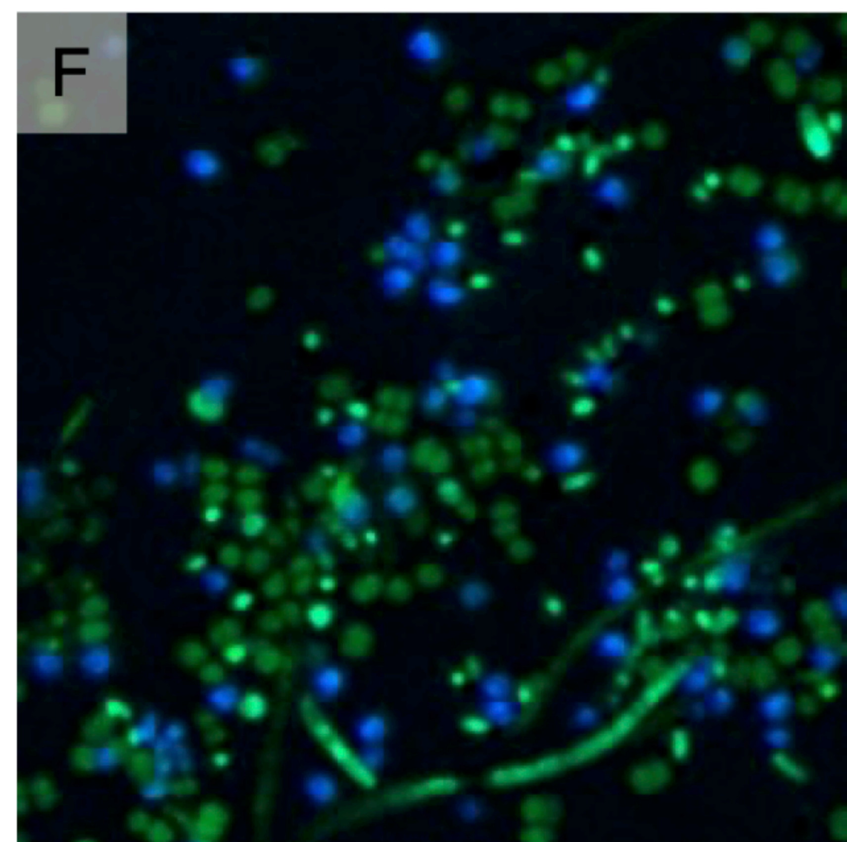
Overlay Verrucomicrobia-Plancto Alphaproteobacteria almost-universal
