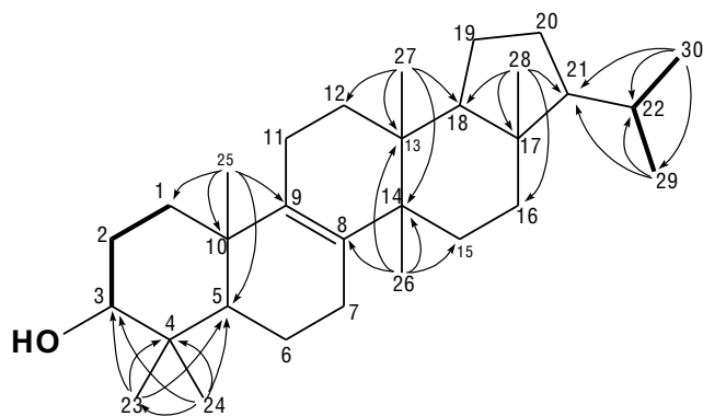
key HMBC (H→C) and 1 H- 1 H COSY (—)Correlations of isomtiol
