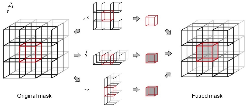
S3 Fig. Sketch of 3D fusion post-processing. An example voxel with red edges in the 3D image is segmented from all three axes. The final 3D label mask is constructed by merging 2D labels in each view. The example voxel is labeled along two axes (y and z, colored in gray) during semantic segmentation, and is thus labeled in the final 3D label mask.
