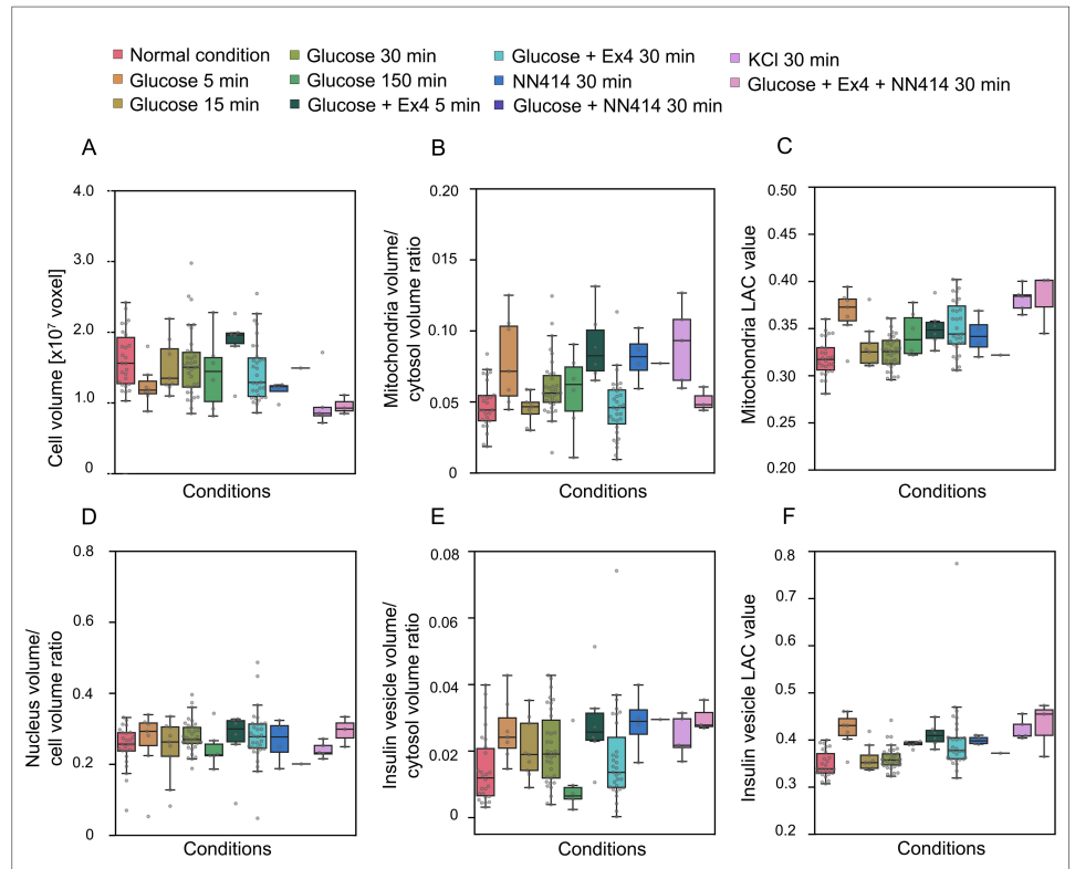
S6 Fig. Comparison of organelles features and localization for all datasets under different conditions. Each feature is compared in one plots. Multi-comparison tests results are listed in S1 Table.
