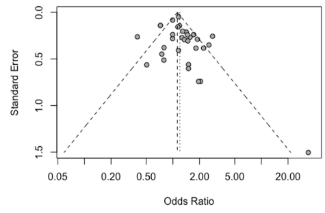
Funnel plot
