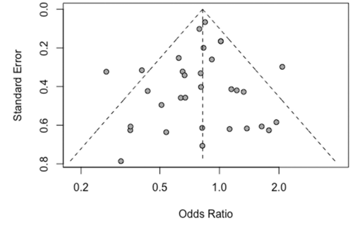
Funnel plot
