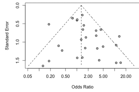
Funnel plot
