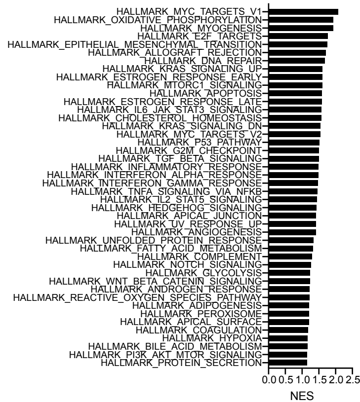
C Hallmark GSEA Positively Enriched in NSG Mice APOBEC Tumors
