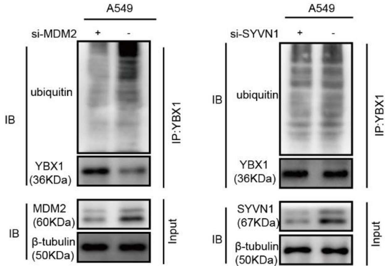
Fig.S1 Knockdown of MDM2 decreased the YBX1 ubiquitination level.
