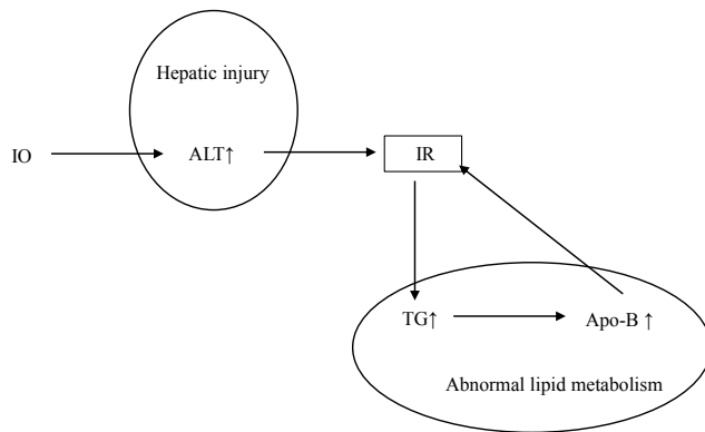
Supplementary Fig. 2. Potential mechanism of insulin resistance (IR) induced by iron overload (IO). The ↑ indicates the increase of the index, while the remaining arrows indicate the facilitation. ALT, alanine aminotransferase; TG, triglyceride; Apo-B, apolipoprotein B.
