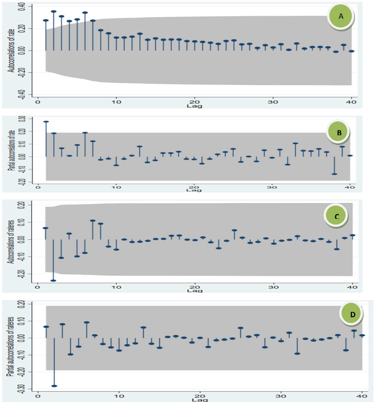
Figure 2: ACF (A, C) and PACF (B, D) plots of U5MR series (A, B), the residual of fitted ARIMA (1,0,4) model (C, D), respectively to predict under five mortality rates in Kersa health and demographic surveillance site, Ethiopia, 2020.
