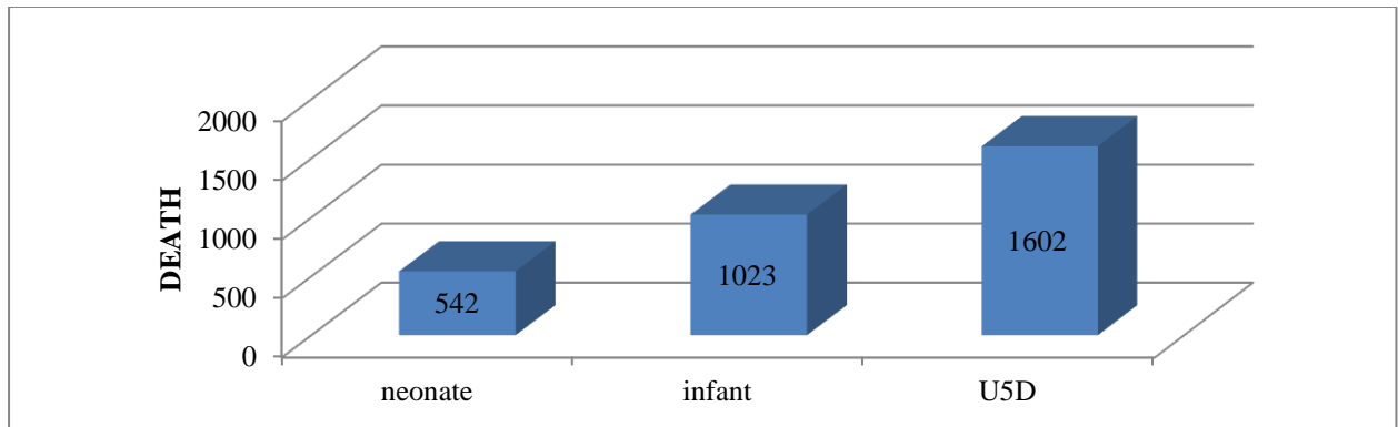
Figure 1: Overall under-five children mortality in Kersa health and demographic surveillance site: 2008-2016 data analysis, Ethiopia, 2020.
