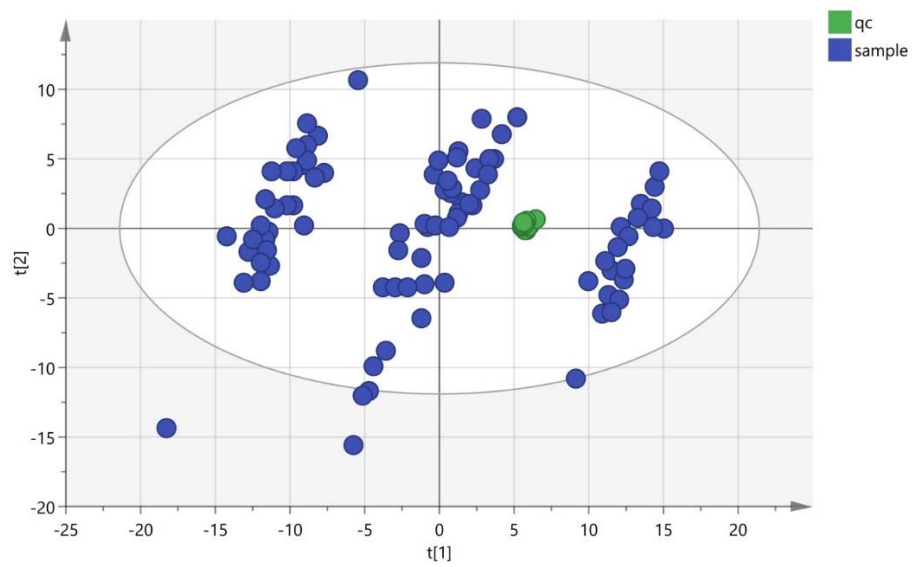
Figure 2 QC result of reversed-phase chromatography anion pattern
