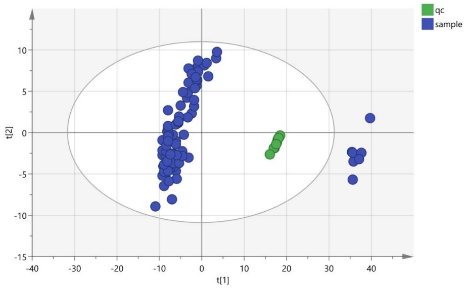
Figure 3 QC result of hydrophilic chromatography positive ion pattern
