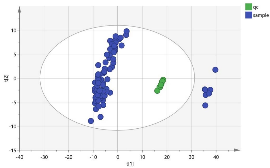
Figure 1 QC result of reversed-phase chromatography positive ion pattern
