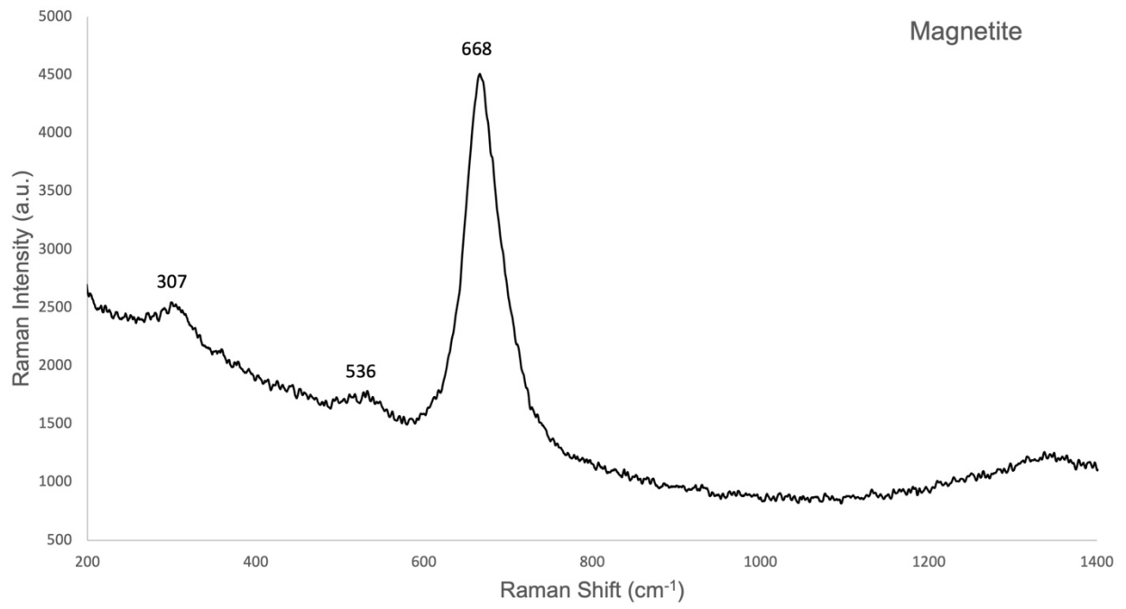
Supplementary Figure S2. Raman spectrum of corrosion product on nail section. Raman spectrum of magnetite in DPL
