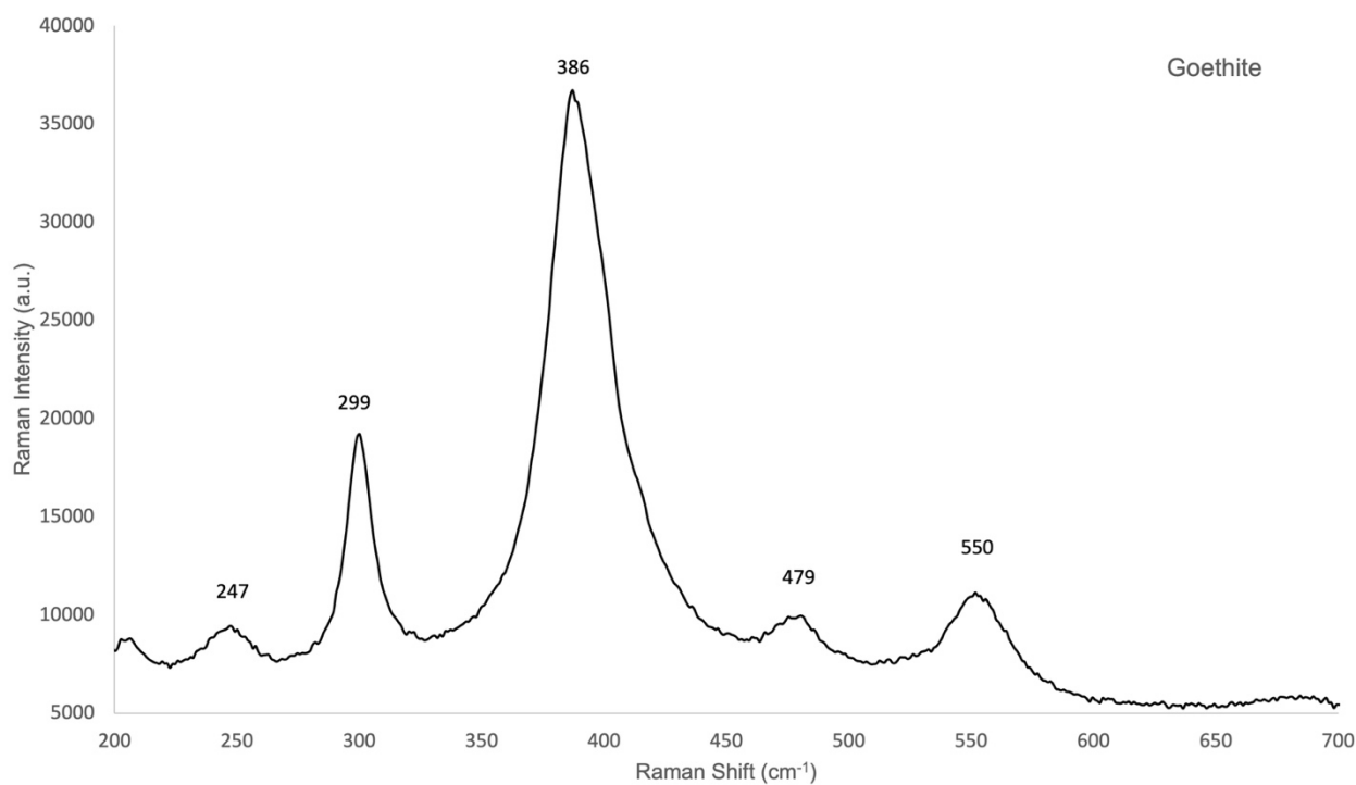
Supplementary Figure S1. Raman spectrum of corrosion product on nail section. Raman spectrum of goethite in DPL
