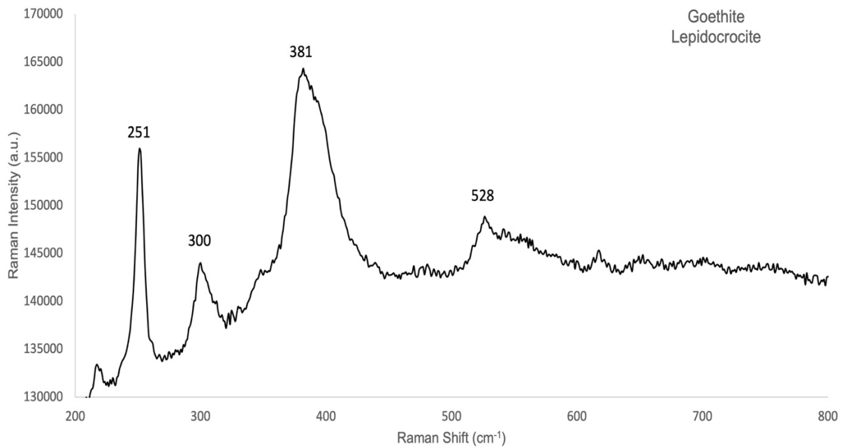
Supplementary Figure S3. Raman spectrum of corrosion product on nail section. Raman spectra of goethite and lepidocrocite in TM
