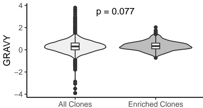
CDR3 Hydrophobicity
