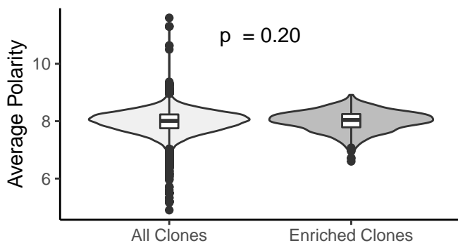
CDR3 Polarity
