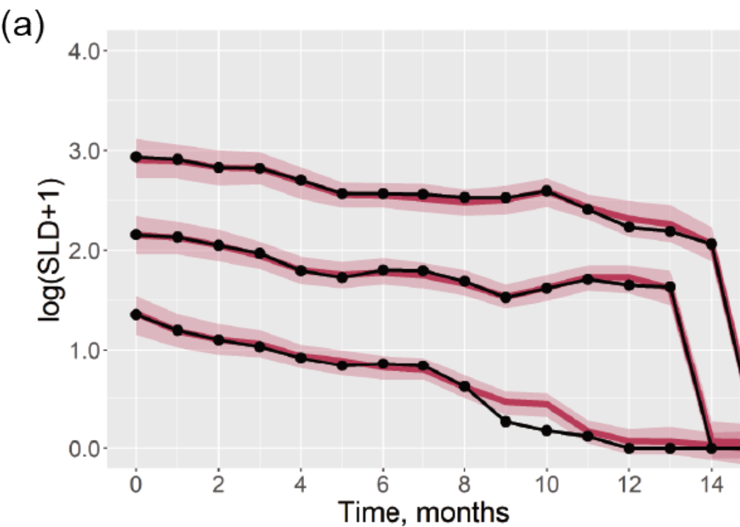
Univariate SLD
