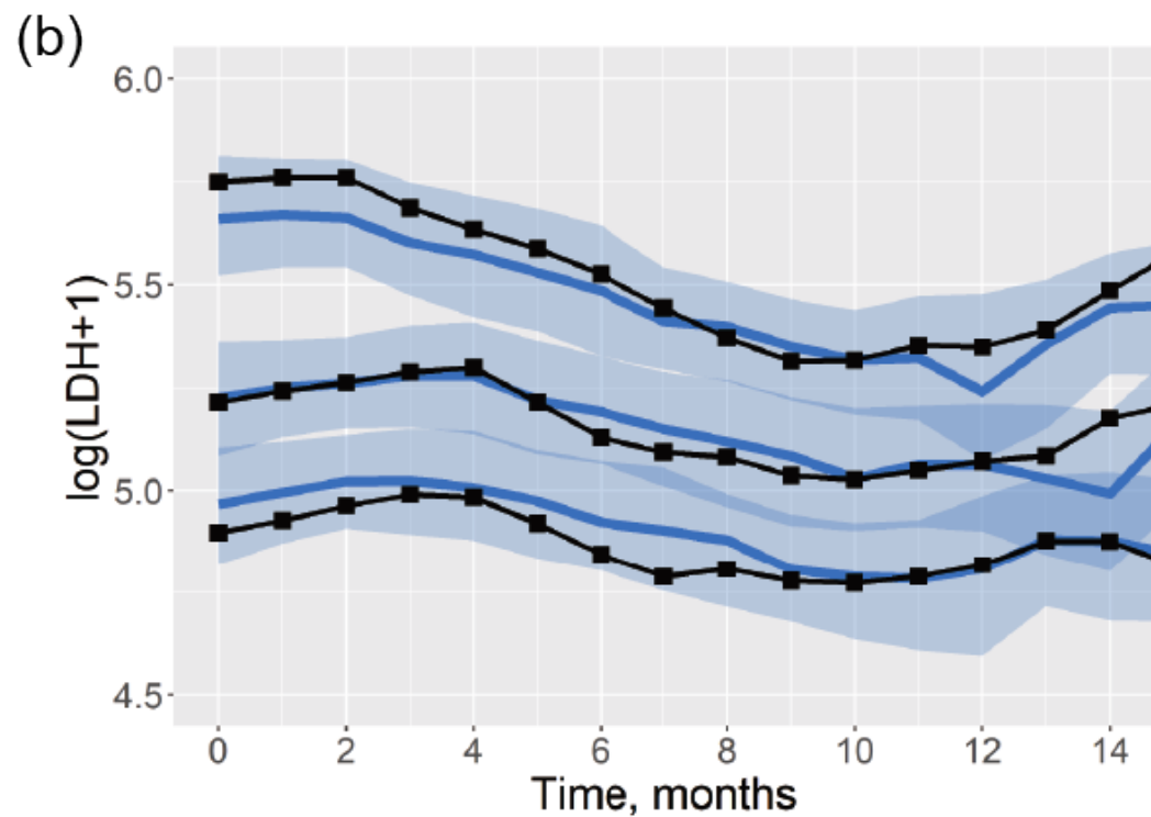
Univariate LDH
