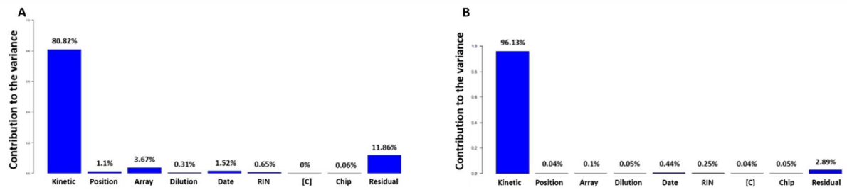
S1 Fig. Data quality by PVCA before and after normalization. Dataset is tested for the presence of technical biases using principal variation component analysis (PVCA). Seven possible sources of batch effect were evaluated, in addition to the ‘kinetic’ biological parameter. Residual is the part of the variance not explained by the different parameters tested ( A ). After normalization, 96.13% of the variance is explained by the kinetic, demonstrating the low impact of technical sources on the dataset ( B ).
