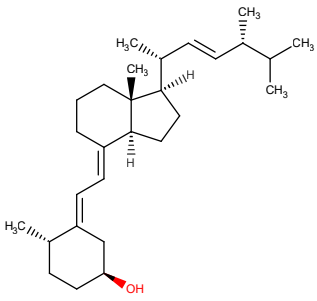
ERGOCALCIFEROL
