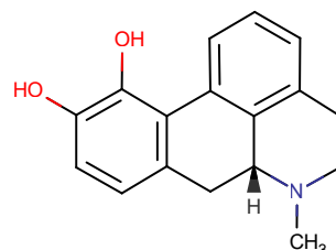
APOMORPHINE
