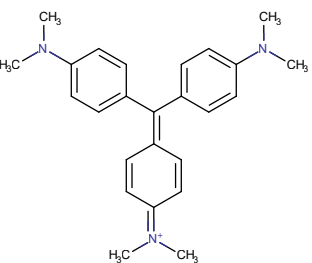
GENTIAN VIOLET
