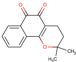
LAPACHONE
