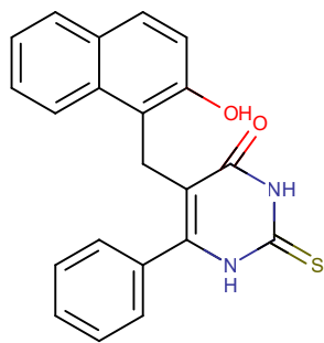
RABEPRAZOLE
