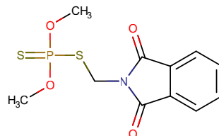
PHOSMET
