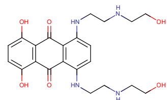
MITOXANTRONE HYDROCHLORIDE
