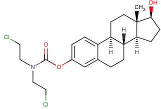
LAPACHONE
