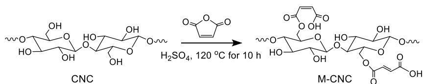
Figure S2 The chemical reaction of MAH modified CNCs surface.
