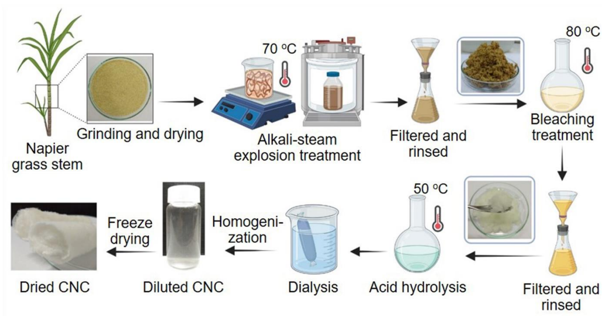
Figure S1. Diagram of the CNC extraction.
