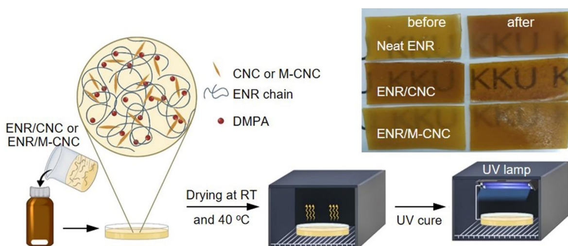
Figure S3. Schematic illustration of the UV-cured nanocomposite preparation.
