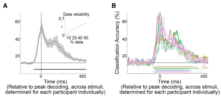
Figure S1. Classification accuracy curves, computed relative to the time-to-peak decoding (corrected)
