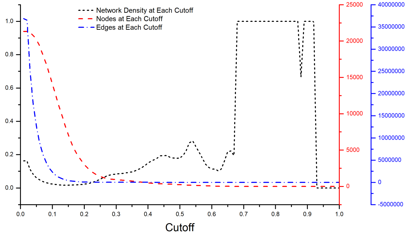
Supplementary Figure S1: Selection of cutoff values. The number of nodes (red), number of edges (blue) and network density are represented as a function of cutoff value. Only edges with value greater than the cutoff value were used to visualize the co-expression network. Only nodes connected by these edges were used in our network analysis. The corresponding network densities at different cutoff values are shown in black dashed line.
