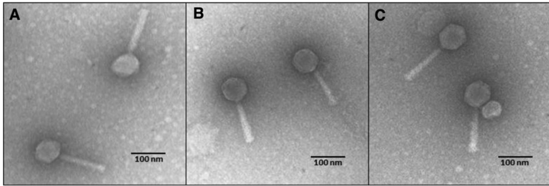
SUPPLEMENTARY FIG. S2. Bacteriophages F8 (A), DP1 (B) and LMA2 (C), TEM imaging. TEM, transmission electron microscopy.
