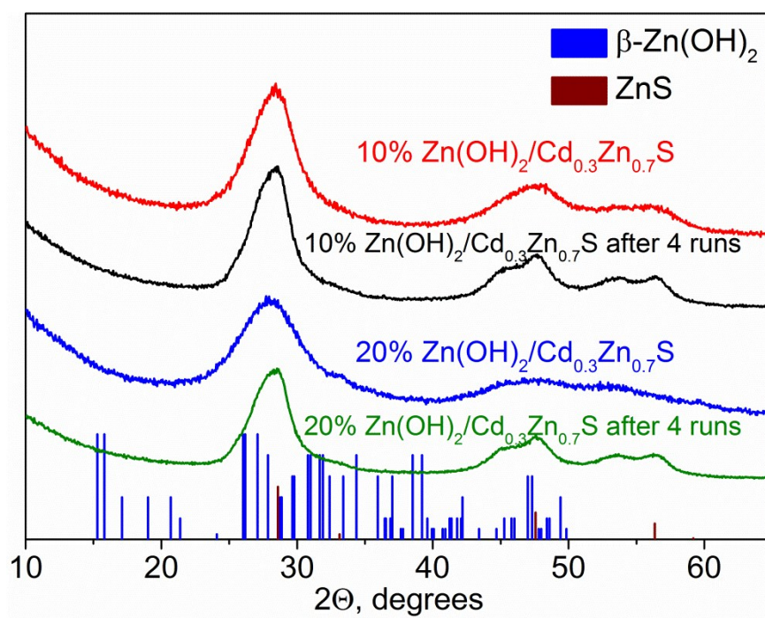
Fig. S1. XRD patterns of 10% Zn(OH) 2 /Cd 0.3 Zn 0.7 S and 20% Zn(OH) 2 /Cd 0.3 Zn 0.7 S before and after photocatalytic hydrogen production from aqueous 0.1 M Na 2 S/0.1 M Na 2 SO 3 solution
