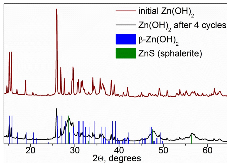
Fig. S2. XRD patterns of blank Zn(OH) 2 before and after photocatalytic hydrogen production from aqueous 0.1 M Na 2 S/0.1 M Na 2 SO 3 solution
