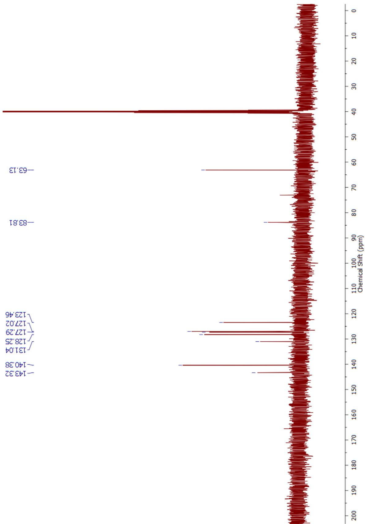
Figure S6: ^{13}\text{C} NMR Spectrum of Compound 4
