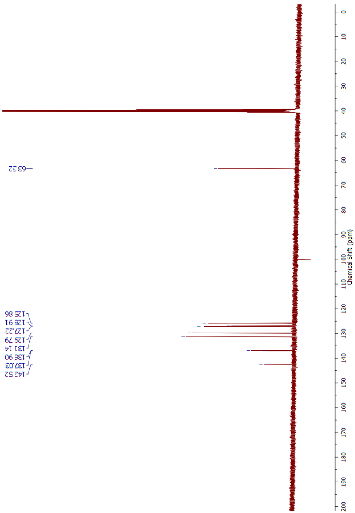
Figure S4: ^{13}\text{C} NMR Spectrum of Compound 3
